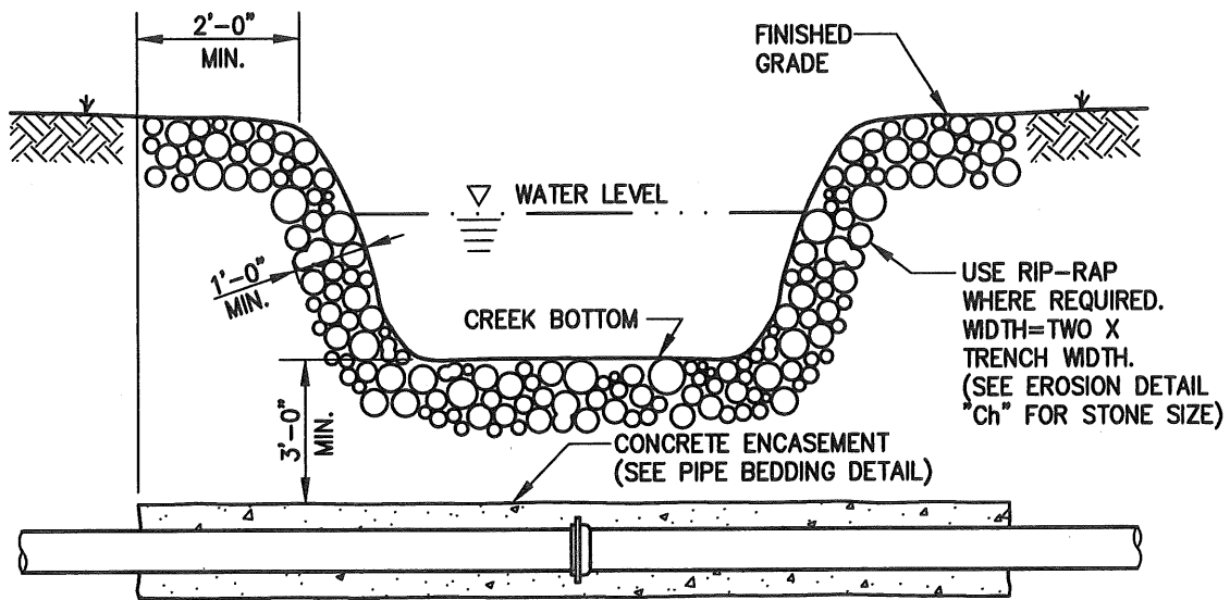
SECTION
