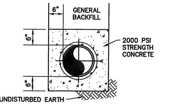
CONCRETE ENCASEMENT
